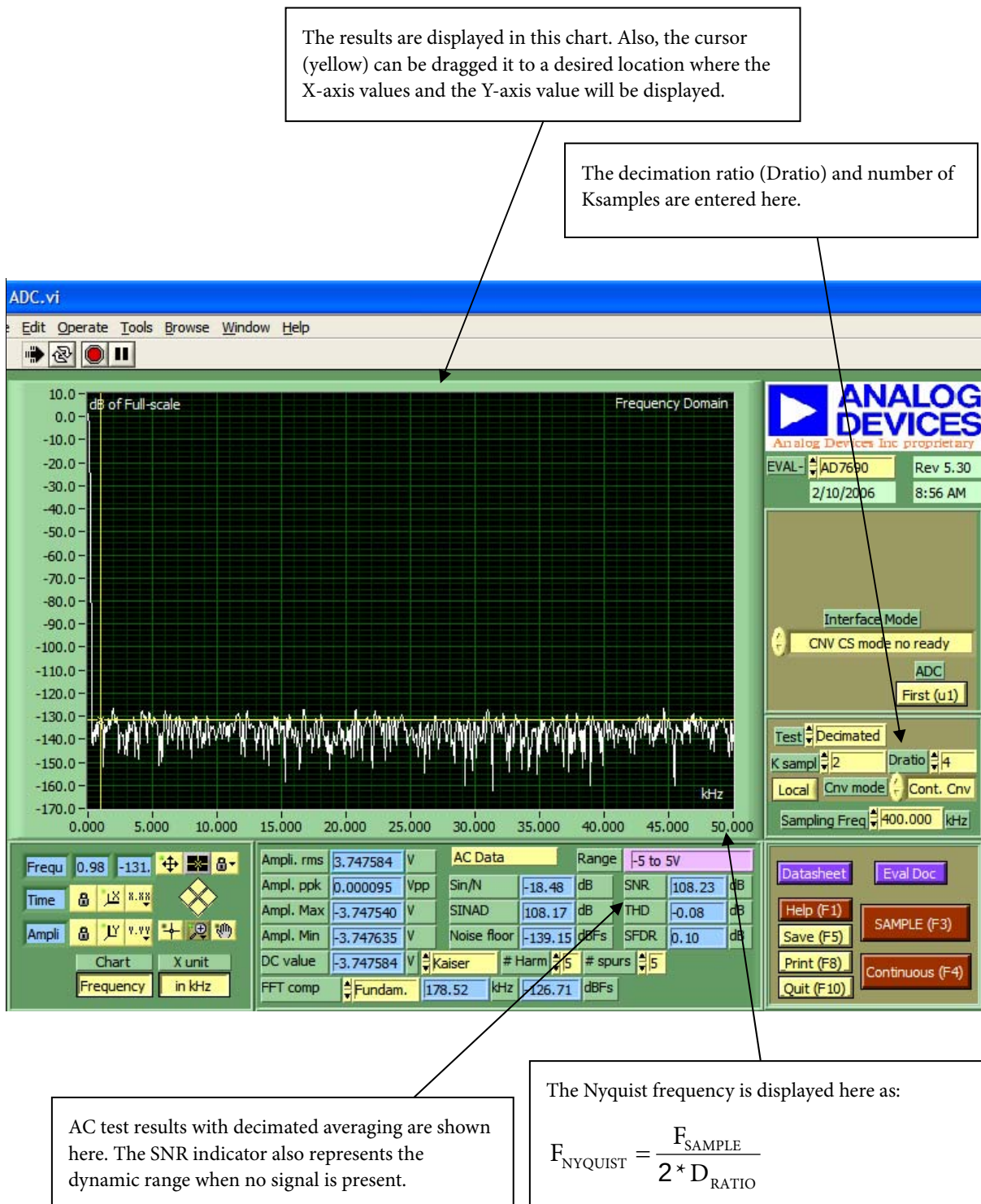
Figure 16. Decimated (Averaging) Screen
